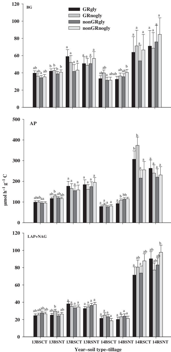
Figure 2. Mean BG, AP and LAP + NAG activities of bulk soil (BS) and rhizosphere soil (RS) associated with conventional tillage (CT) and no-till (NT) and the following treatments: GR corn with and without glyphosate (gly, nogly) applications (GRgly, GRnogly), and non-GR isogenic cultivar with and without glyphosate applications (nonGRgly, nonGRnogly) in 2013 and 2014. Different letters above error bars associated with treatments per sampling year 13,14 and soil type by tillage indicate differences at P < 0.05 .
